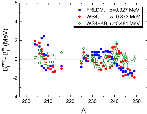
Fig. 4. (color online) The same as Fig. 2(a), but with the results of the finite-range liquid-drop (FRLDM) model [25] and B_f^{\text{WS4}} + \Delta B for comparison. The error bars denote the difference between the inner barrier height and the corresponding outer barrier height for actinides [3].
