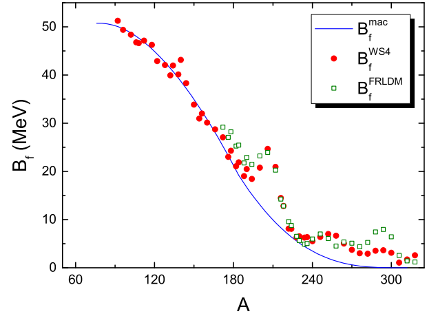
Fig. 5. (color online) Fission barrier heights for even-even nuclei which lie on or are the closest to the \beta -stability line (using Green's expression [37]).
